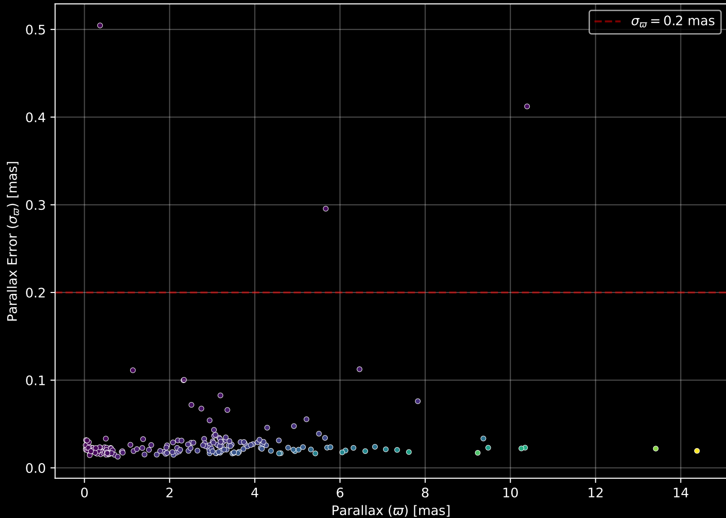
APOGEE DR17 Field: [279+66] Parallax Quality (n= 191)
