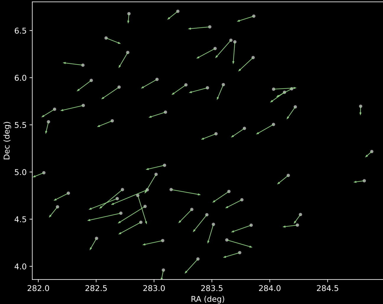
APOGEE DR17 Cluster 5 Proper Motion Vectors (n=60)
