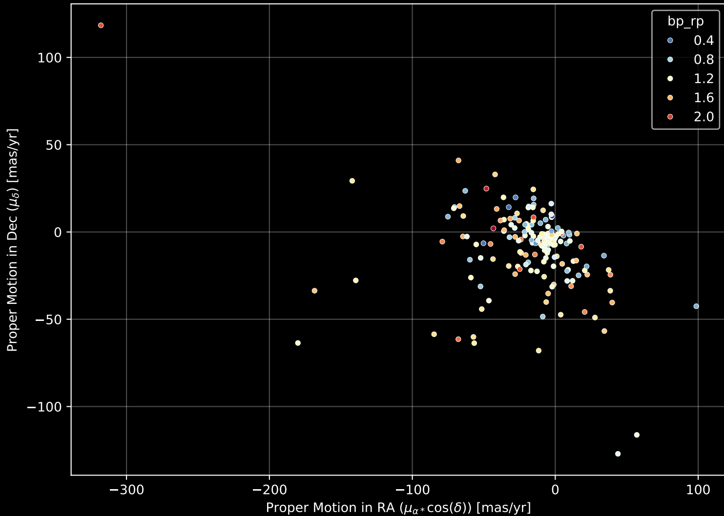
APOGEE DR17 Field: [279+66] Proper Motion Diagram (n= 191)
