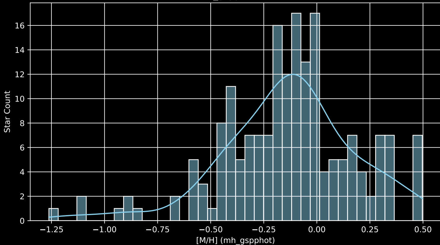
APOGEE DR17 Field: [279+66 [M/H] (mh_gspphot) (n= 186)
