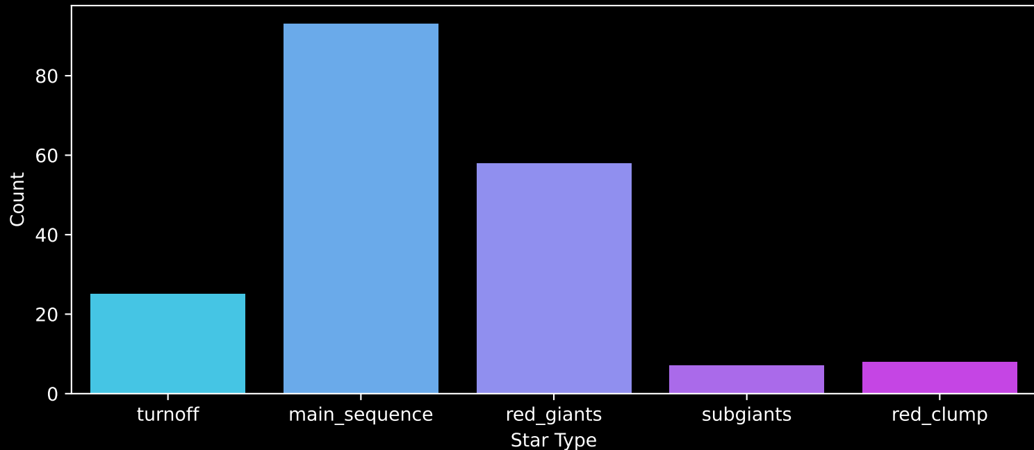
APOGEE DR17 Field: [279+66] Count plot of Star Type
