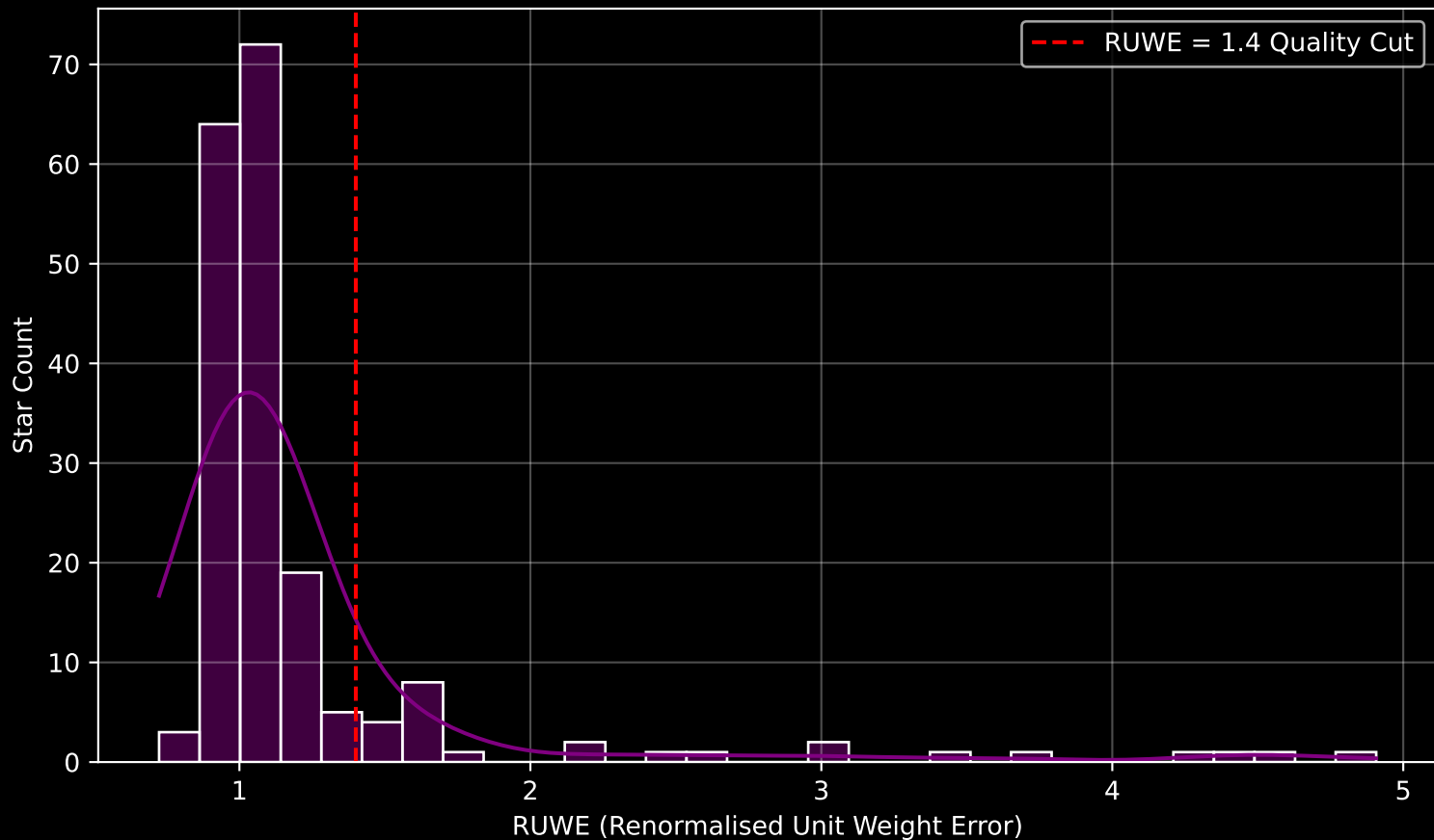
GAPOGEE DR17 Field [279+66] RUWE Distribution (n= 188)
