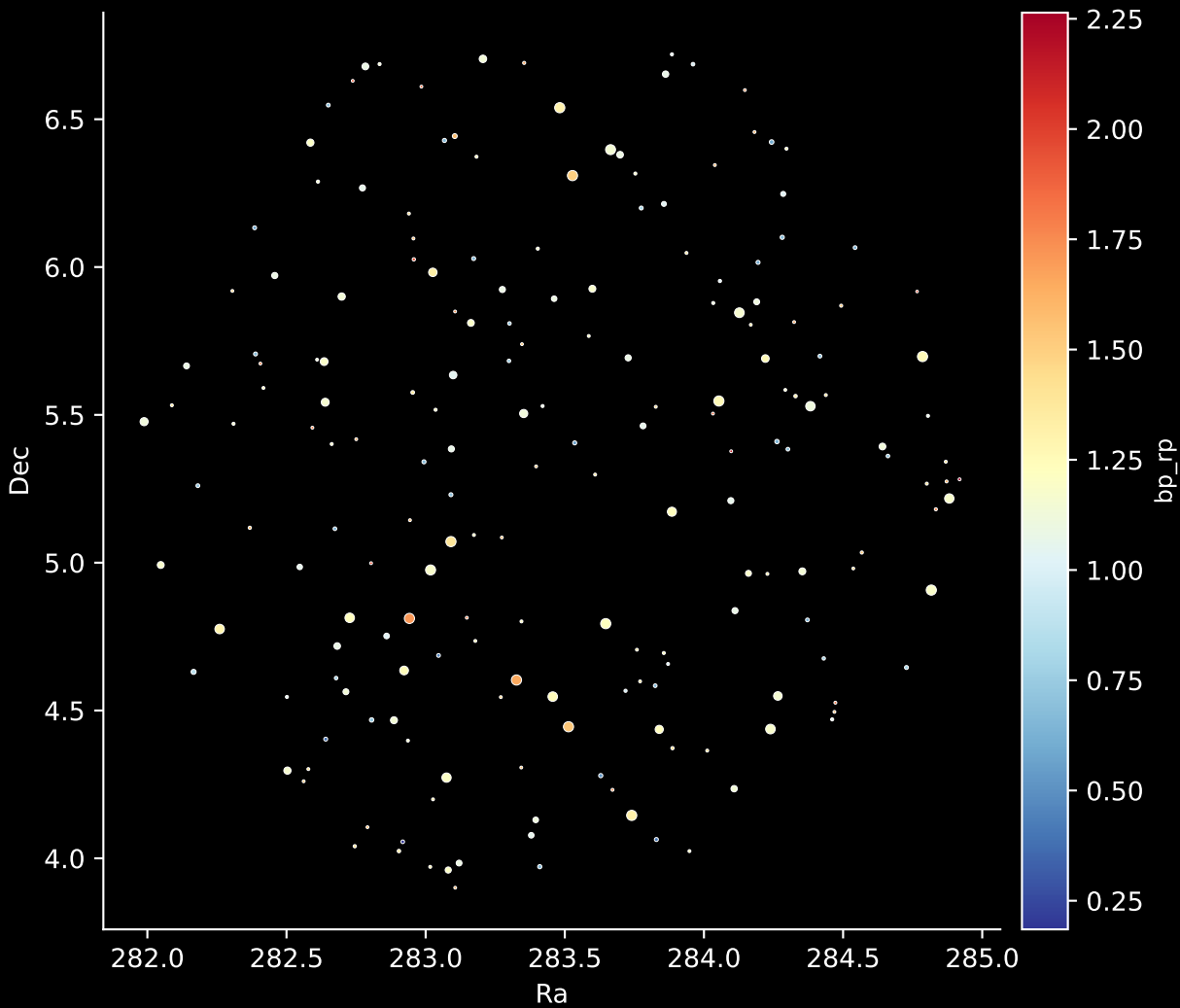
APOGEE DR17 Field: [279+66] Stars: 191
